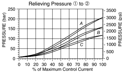
Typical Relief Pressure vs. Flow Characteristic Typical Relieving Pressure ① to ② at Various %'s of Maximum Control Current Pressure Range "A" (207 bar/3000 psi); Cartridge in Body
